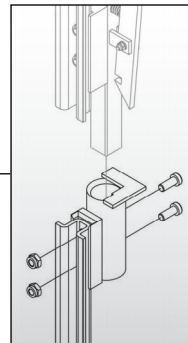
Kupplungsstück H-50 Standard Coupling piece H-50 standard
